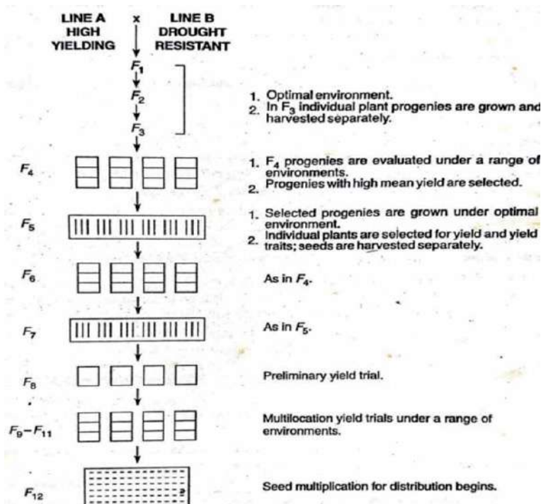
Figure 2. A breeding approach to develop drought resistant variety for different environmental conditions.
