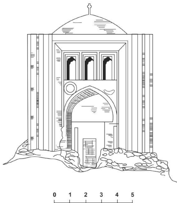
4-rasm. Maqbaraning bosh fasadi – kirish portali.
