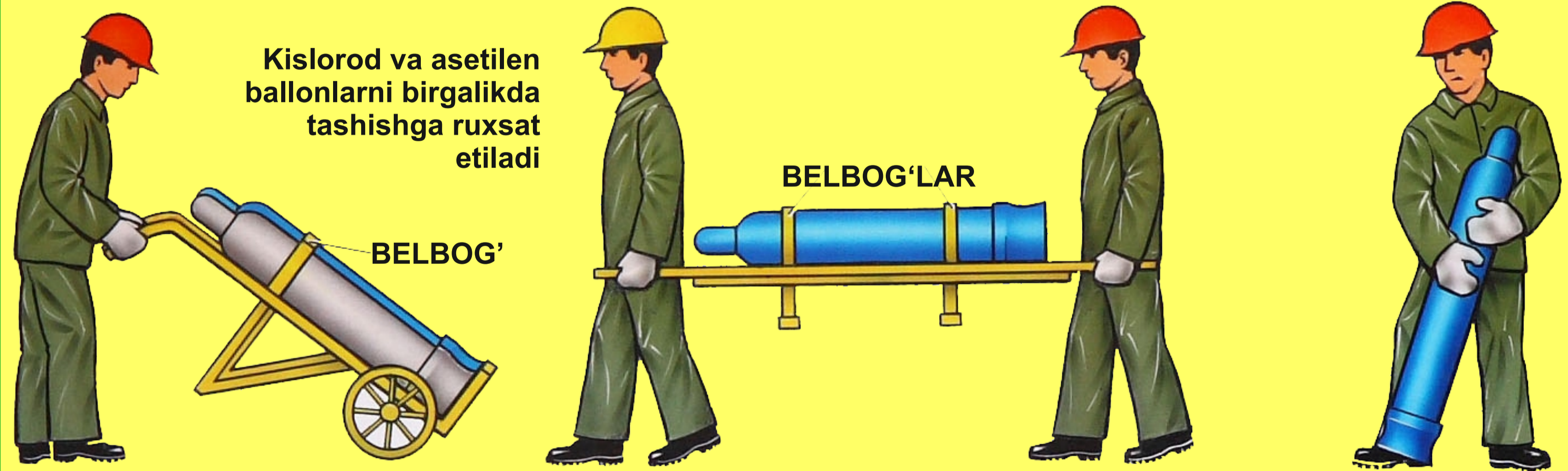
MAXSUS ARAVALAR YORDAMIDA MAXSUS ZAMBILLAR YORDAMIDA QIYA AYLANTIRGAN HOLDA
